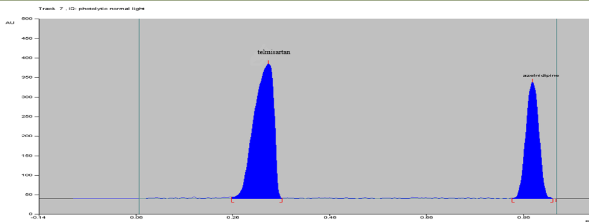
Figure 5. Chromatogram of azelnidipine and telmisartan sample subjected photo degradation (AZL= 0.80, TLM =0.25)
